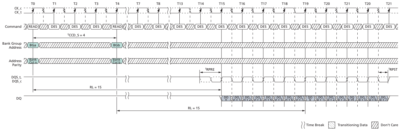
Figure 148: Consecutive READ (BL8) with 1 st CK Preamble and CA Parity in Different Bank Group
